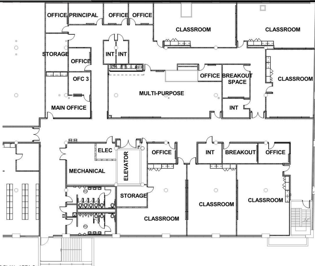
FIFTH FLOOR PLAN - AREA C
