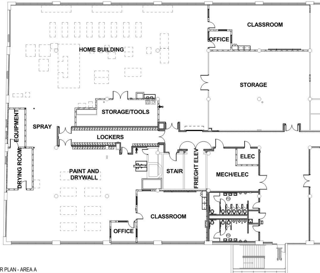
FIFTH FLOOR PLAN - AREA A
