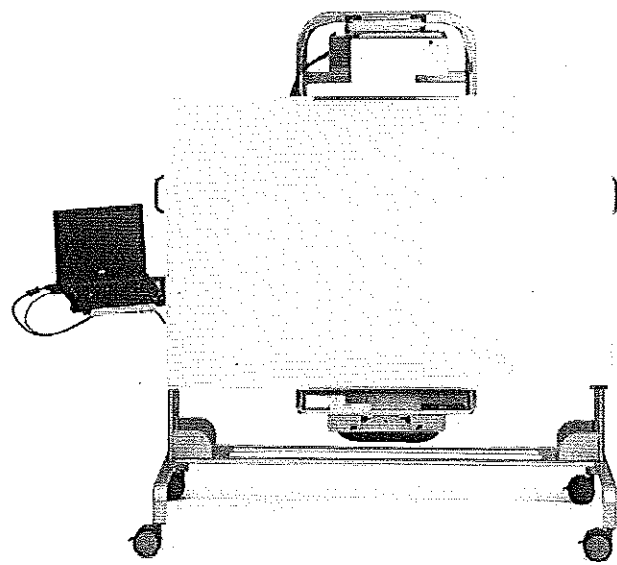
The Mobile Interactive Whiteboard is height adjustable for use by children or adults and can fit through a 32"W doorway.
